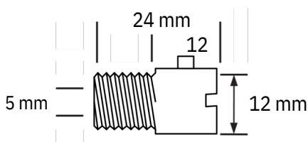
Bayonet Adaptor, Single Pin 1/8" BSP Tapered Thread
